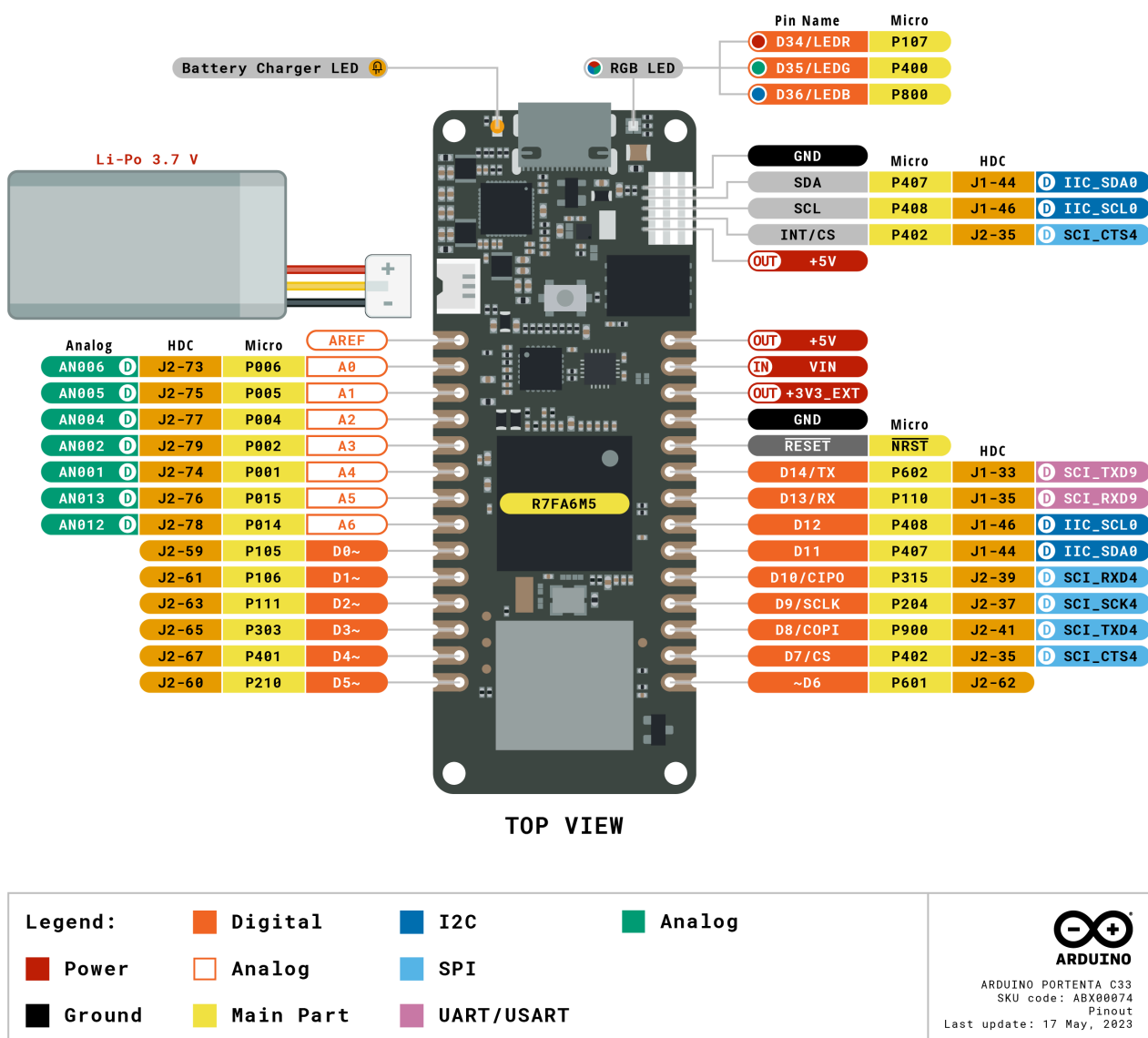
Figure 1. Portenta C33 pinout (MKR-styled connectors)
